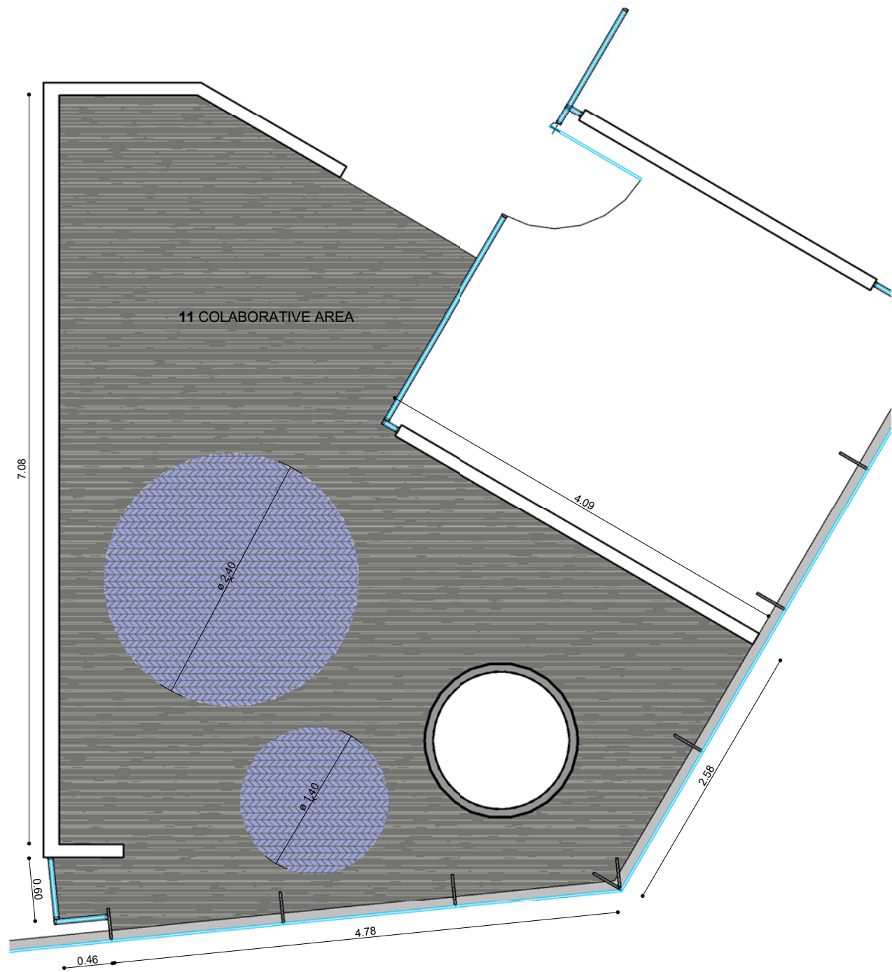
SECTOR A REFORMAR 3 1:100
