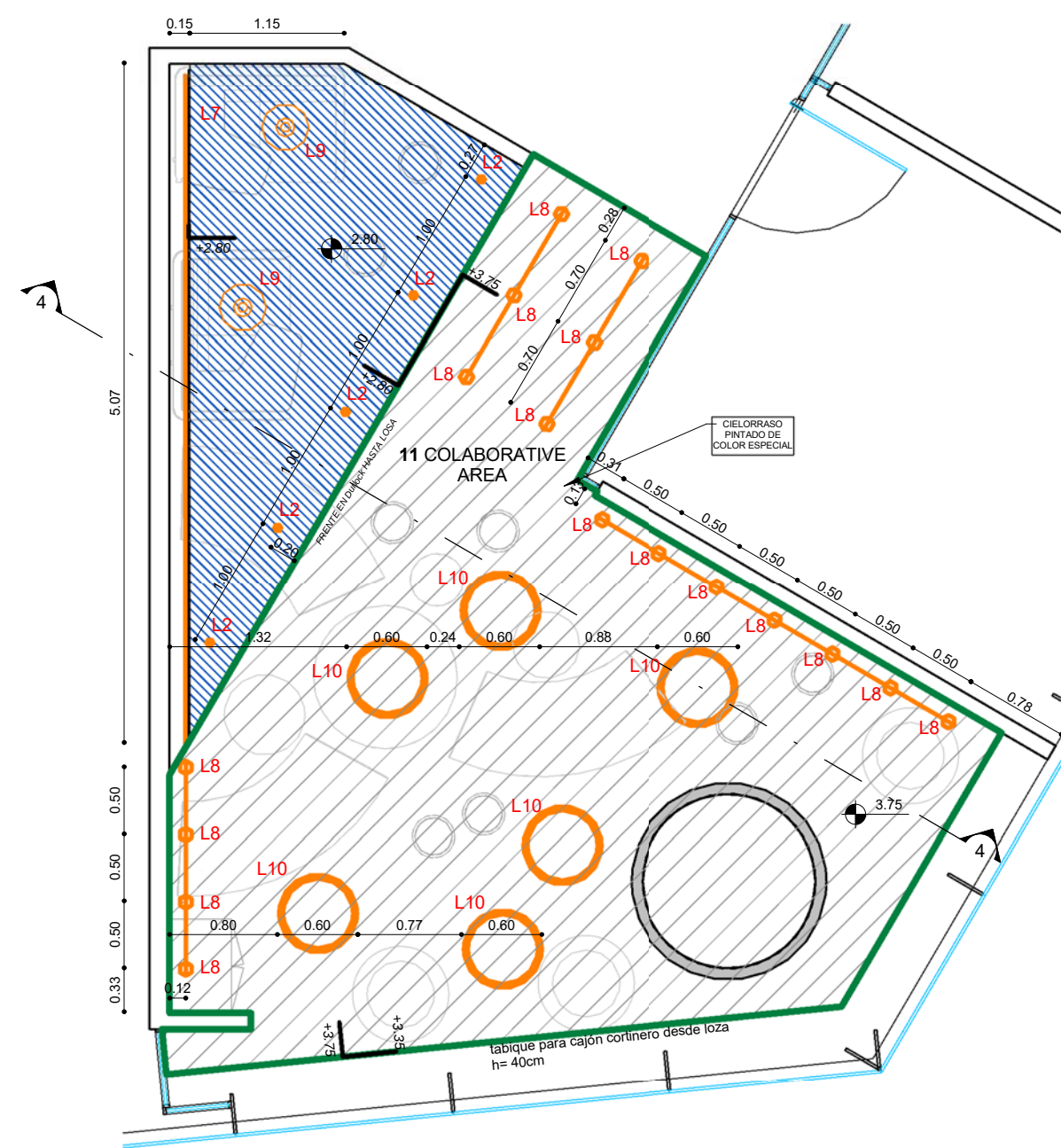
SECTOR A REFORMAR 3 1:50
