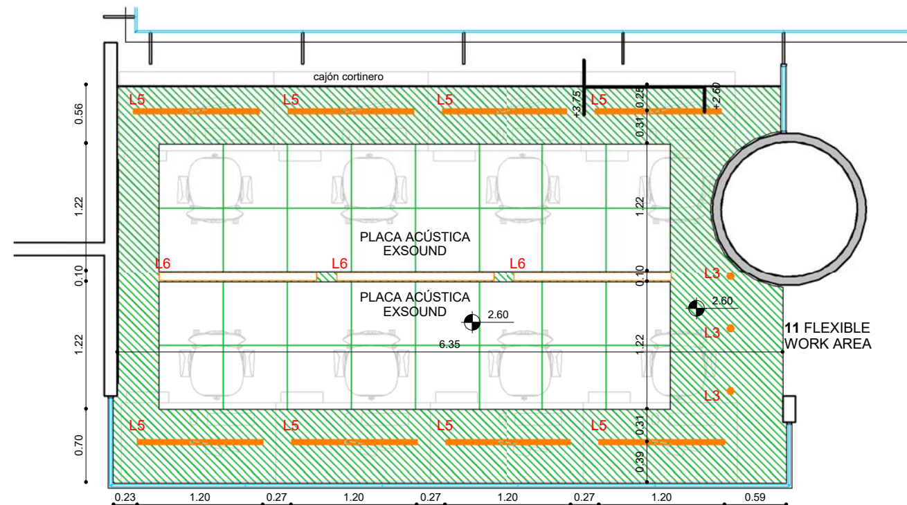
SECTOR A REFORMAR 2 1:50
