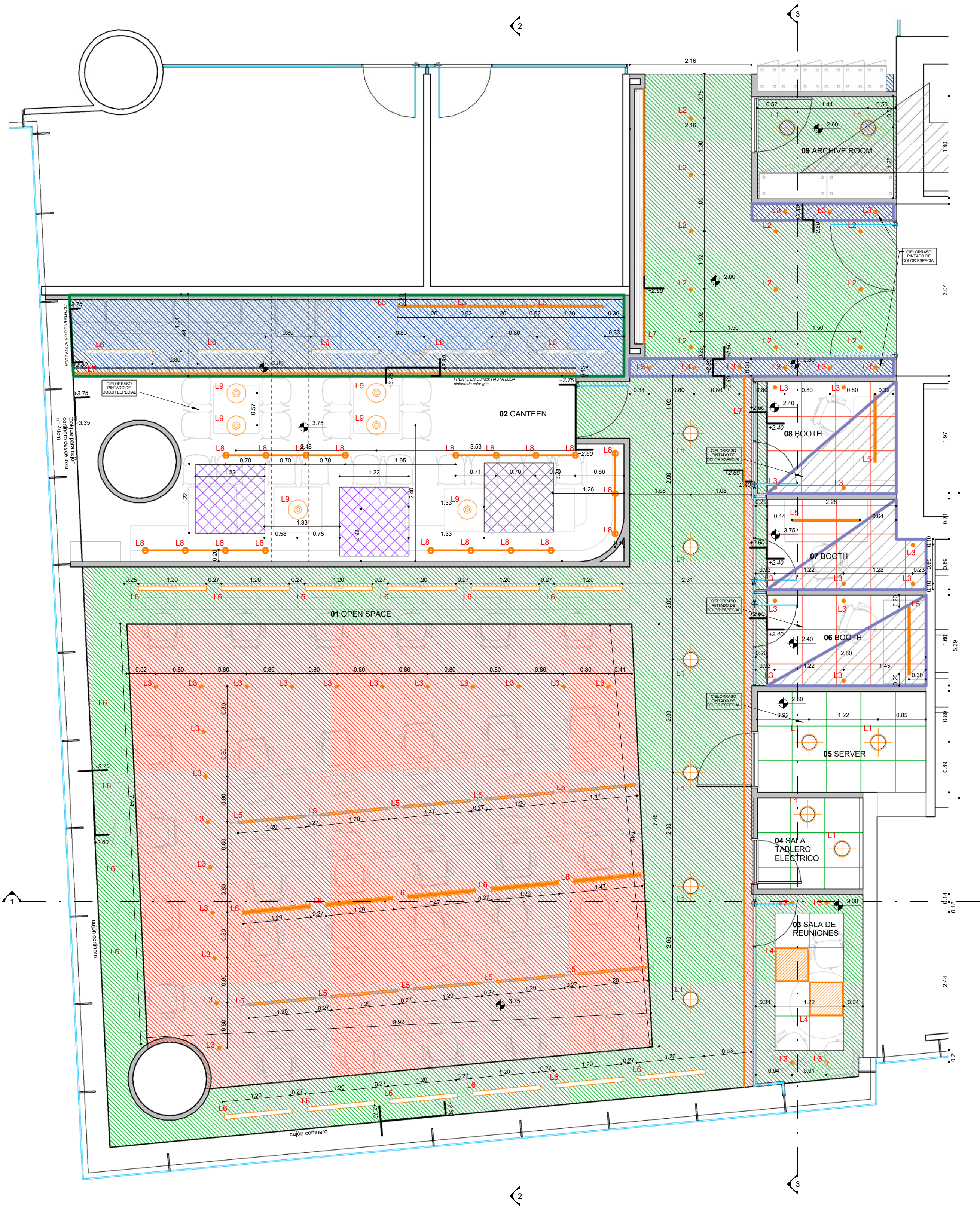
SECTOR A REFORMAR 1 1:50
