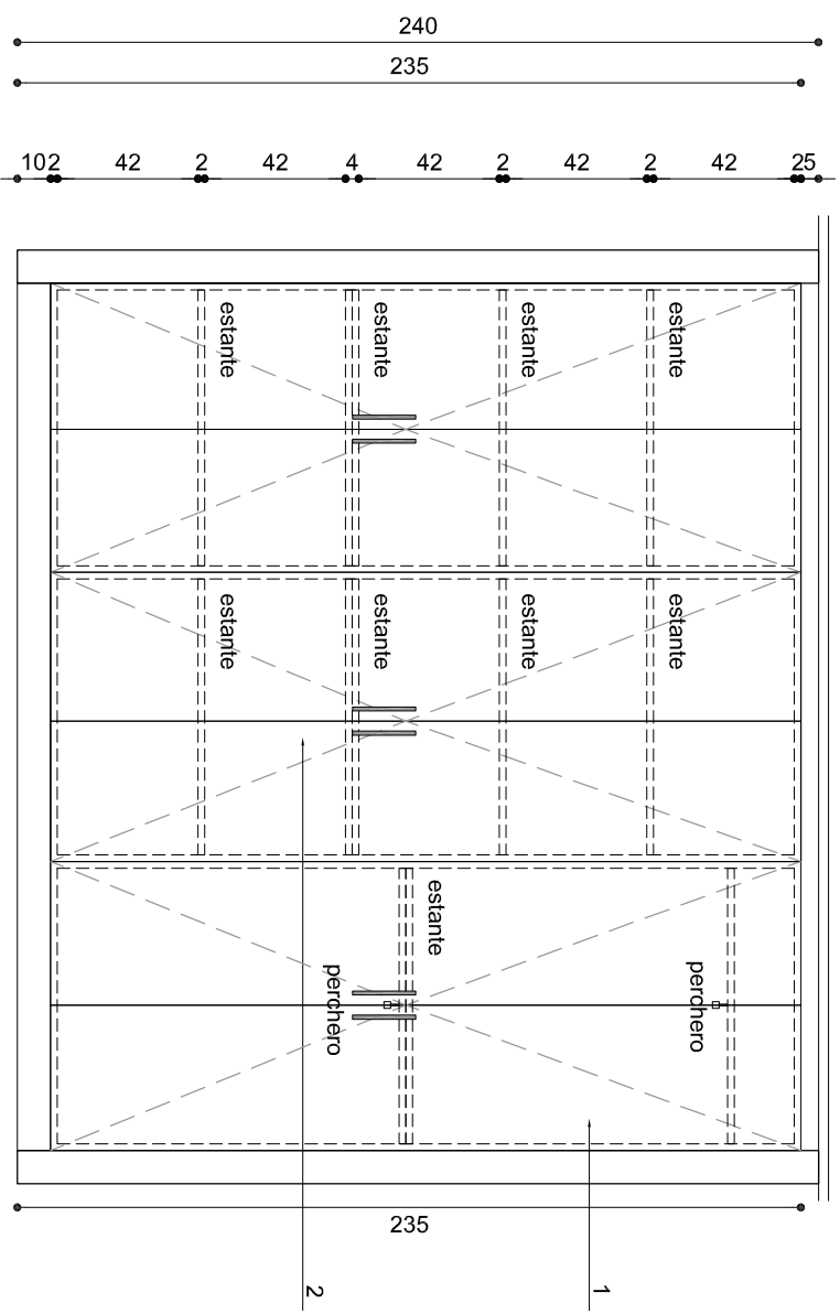
VISTA FRONTAL
