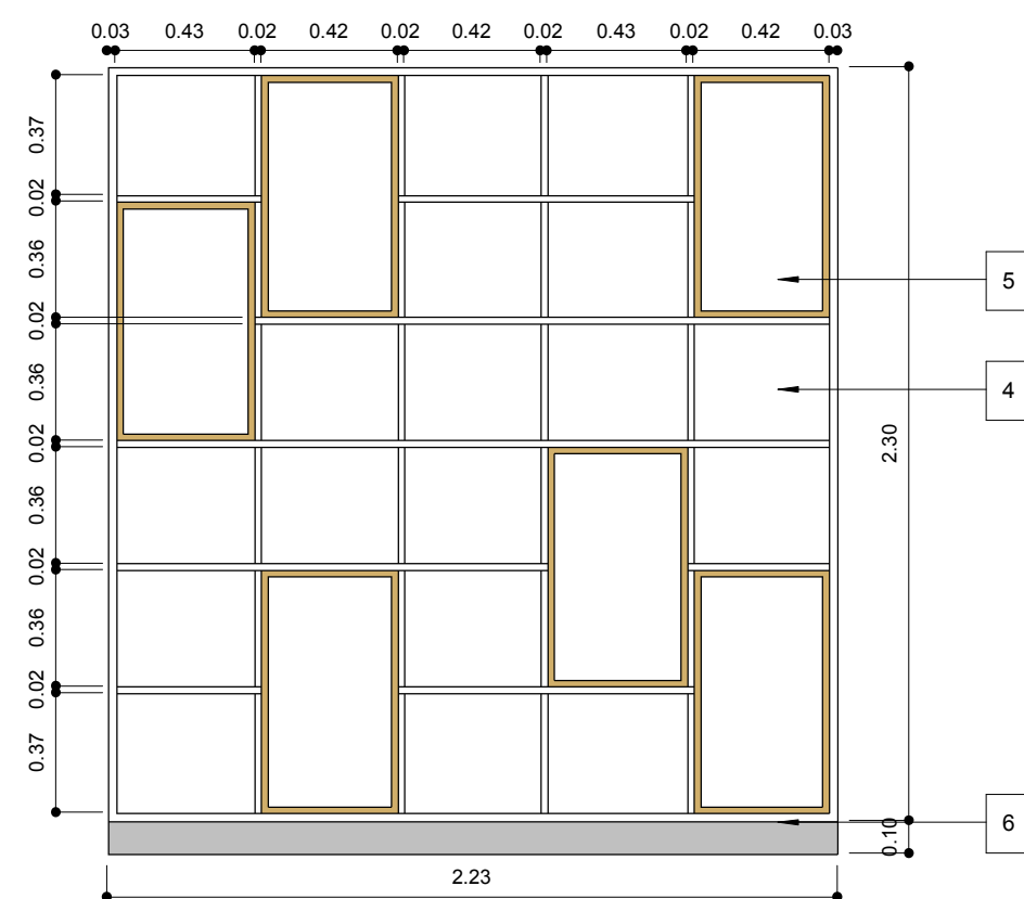
VISTA SHOWROOM 1 : 25
