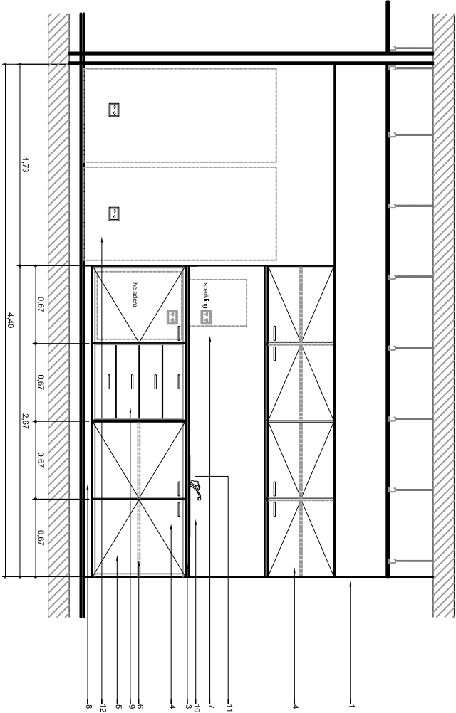
VISTA FRONTAL 1
